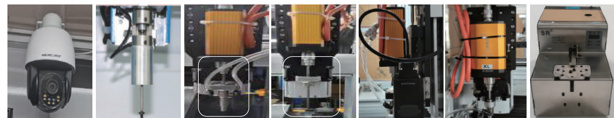
360度攝像錄影手機遠程監控 360-degree camera recording and mobile remote monitoring 電磁磁(螺絲機專用) Electric magnetic (special for screw machine) 真空吸嘴式 Vacuum nozzle type 磁吸式批頭入孔 Magnetic head entry hole 掃碼槍 Barcode scanner 伺服智能電批 servo intelligent batc 吸附式供料器 Adsorption feeder
